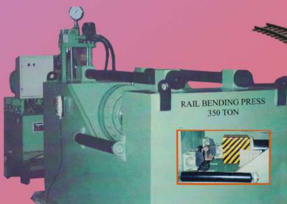
RAIL BENDING PRESS
